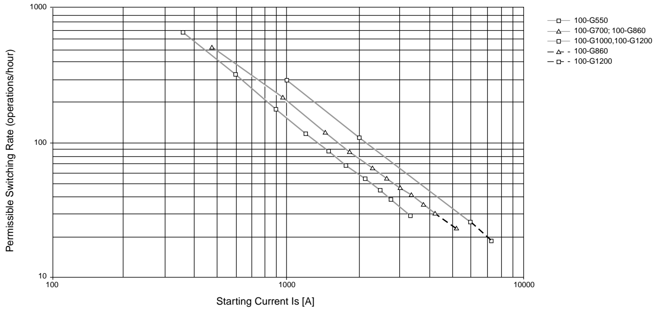
Figure 41 - Switching of Starting Motors (AC-2, and AC4) U_z = 380...460V AC; Starting Time t_{ed} = 1 s, ( <t_s )
