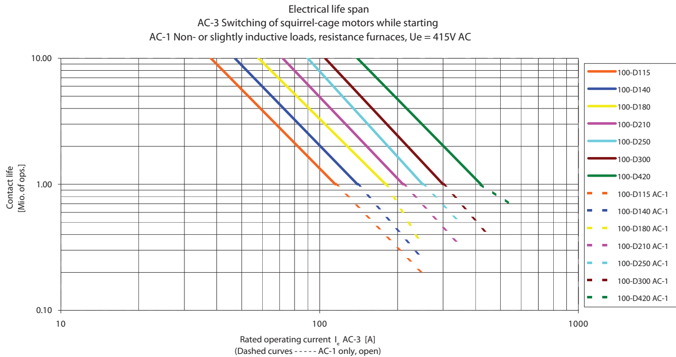
Figure 27 - AC-3, AC-1
