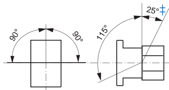
Figure 32 - Mounting Position, 100S-D Contactors
