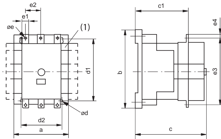
Figure 30 - Bulletin 100-D/100S-D Contactors and Accessories
