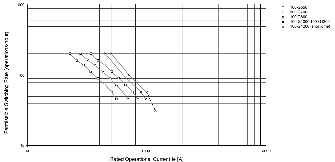
Figure 40 - Switching of Running Squirrel-cage Motors AC-3, U_e = 380...460V AC; Starting Time t_s = 1 s, Relative Running Time 40%
