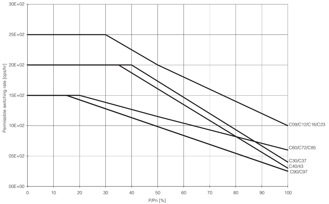
Figure 13 - AC-1, 40 °C Non- or slightly inductive loads, resistance furnaces; U_e = 230...690V
