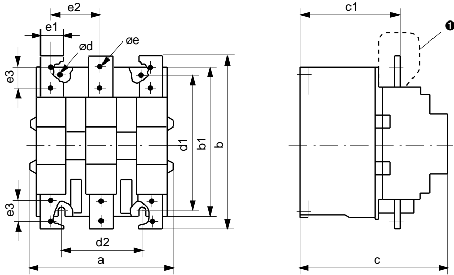
Figure 43 - Mounting Position
