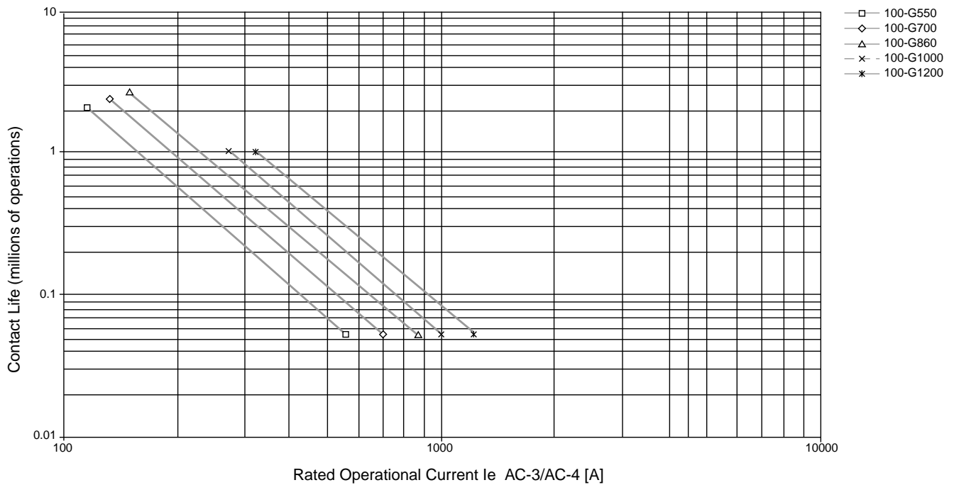
Figure 38 - AC-3 90% Switching of Running Motors, U_e = 380...460V AC; AC-4 10% Jogging
