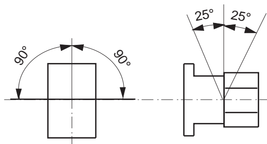
Figure 32 - Mounting Position, 100S-D Contactors
