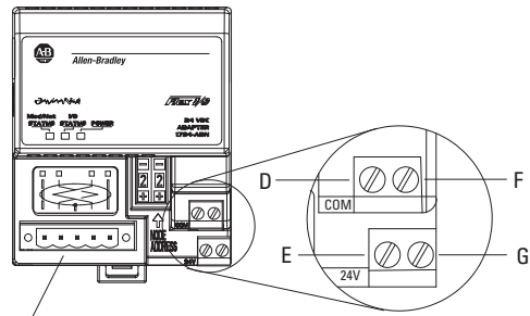
DeviceNet Connector
