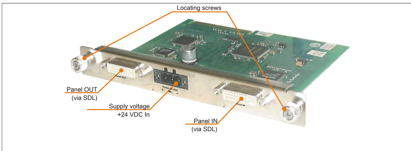
Figure 84: 5DLSDL.1000-01 - Interfaces
